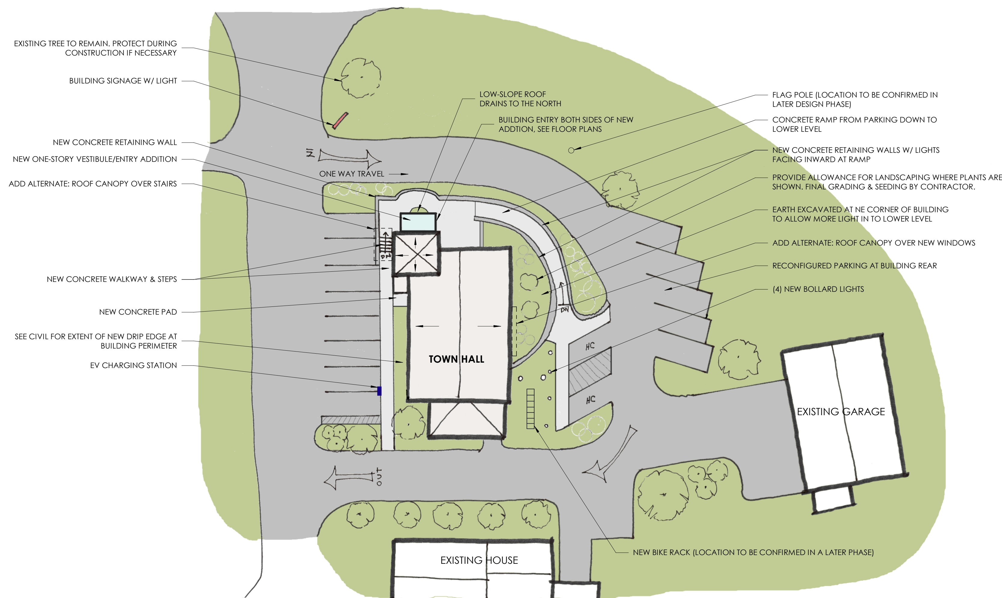
1 Site Plan- Option A 1" = 20'-0"
